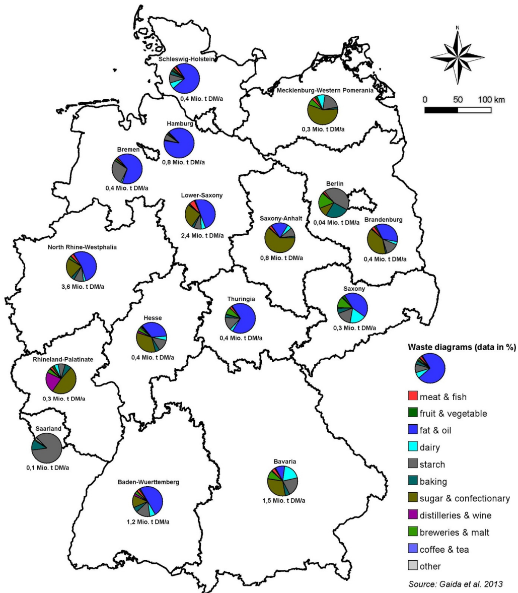
Figure 1. National waste streams of the different FAB industry branches in each federal state
